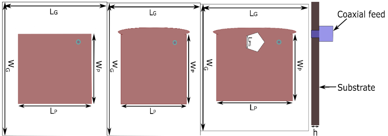
Fig.2. Evolution of proposed Antenna a)Antenna1 b) Antenna2 c) Antenna3 (proposed) d)Side view
