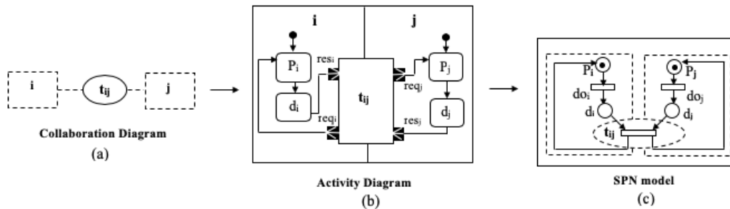
Fig.7. SPN model of a collaboration
